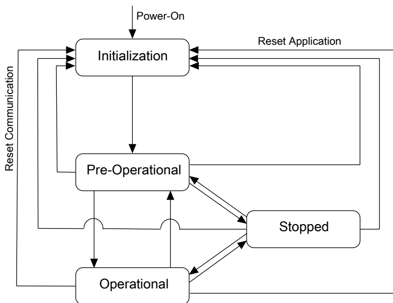
Abb. 1: NMT ( http://doc.ingeniamc.com/emcl2/command-reference-manual/communications/canopen-protocol/canopen-objects/nmt/nmt-state-machine ), abgeändert
