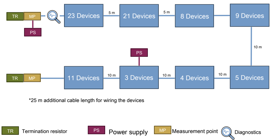
Fig. 36: 500 kbit/s, 84 devices, cable length 75 m
