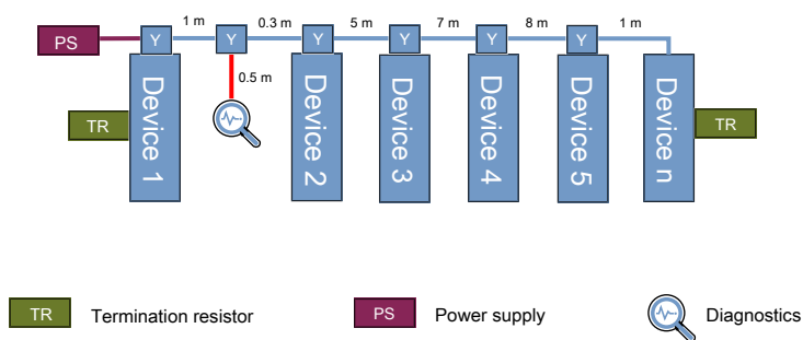
Fig. 25: Network with Y-connectors
