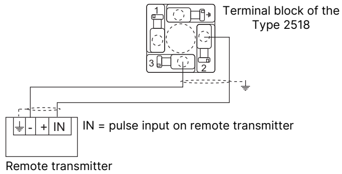
Fig. 10: Wiring of the sinus output of a sinus version
