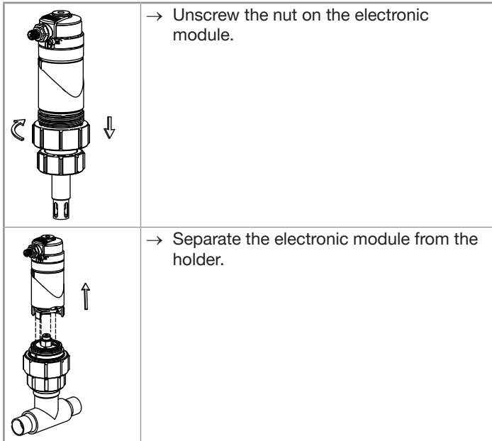
Fig. 23: Replacing the seal in the probe holder
