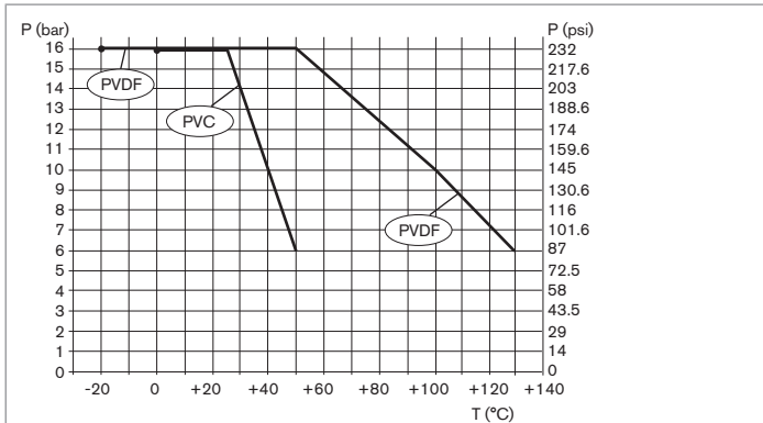
Fig. 3: Dependency between the fluid temperature and the fluid pressure, device variant with a PVC nut or device variant with a PVDF nut, without probe
