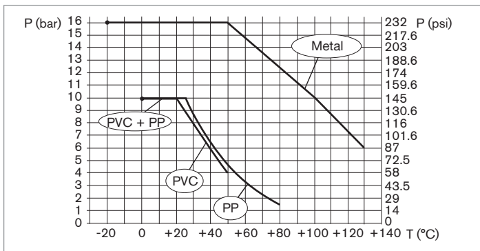
Fig. 5: Dependency between the fluid temperature and the fluid pressure, device variant with a PVDF nut, without probe, with a Type S022 in metal, PVC or PP
