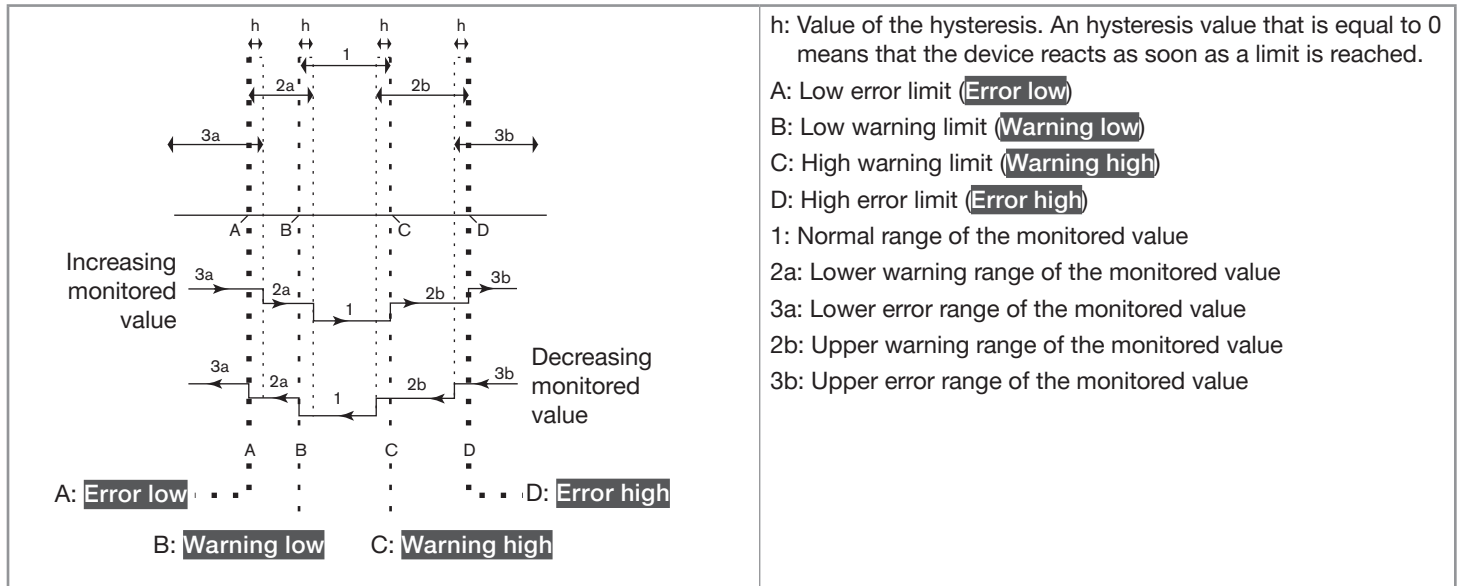
Fig. 16: Operating principle of the monitoring with an hysteresis
