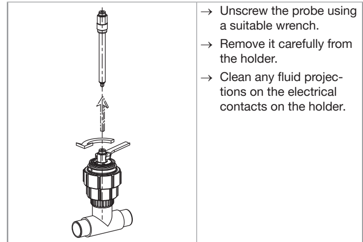
Fig. 22: Removing the probe from the holder
