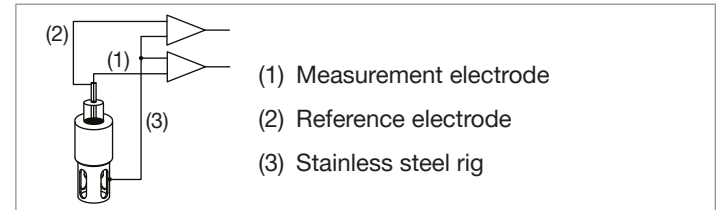
Fig. 14: Schematic diagram of symmetrical measurement
