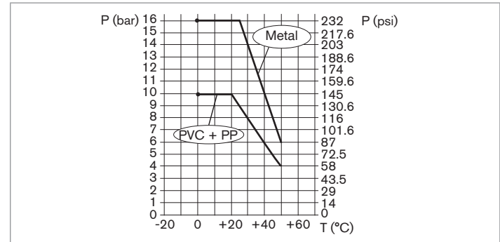
Fig. 4: Dependency between the fluid temperature and the fluid pressure, device variant with a PVC nut, without probe, with a Type S022 in metal, PVC or PP
