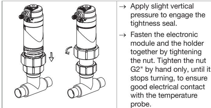
Fig. 13: Fitting the electronic module to the holder
