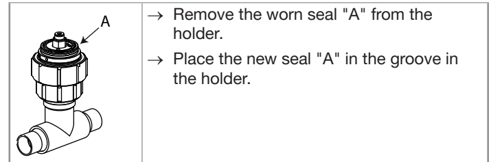
Fig. 23: Replacing the seal in the probe holder
