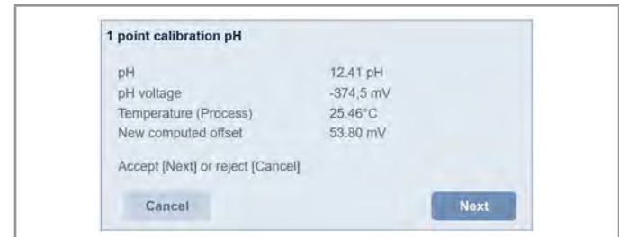
Fig. 20: Validation screen of the pH calibration procedure
