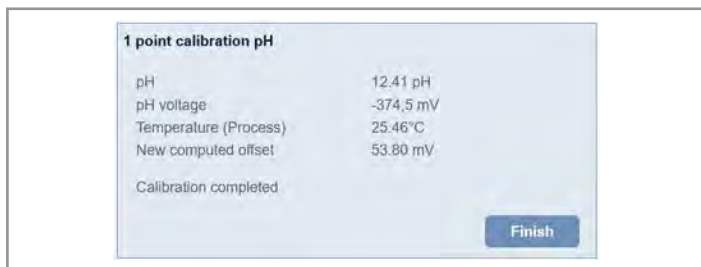
Fig. 21: Final screen of the pH calibration procedure
