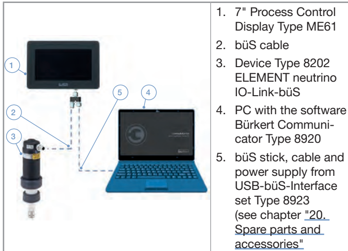
Fig. 17: Example of arrangement for setting the calibration action on the 7" Process Control Display Type ME61
