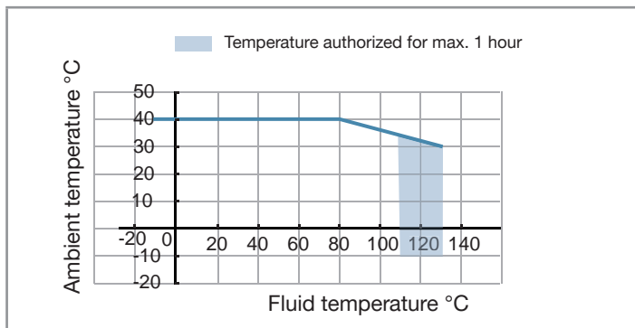
Fig. 2: Fluid temperature depending on the ambient temperature for an ATEX or an IECEx product
