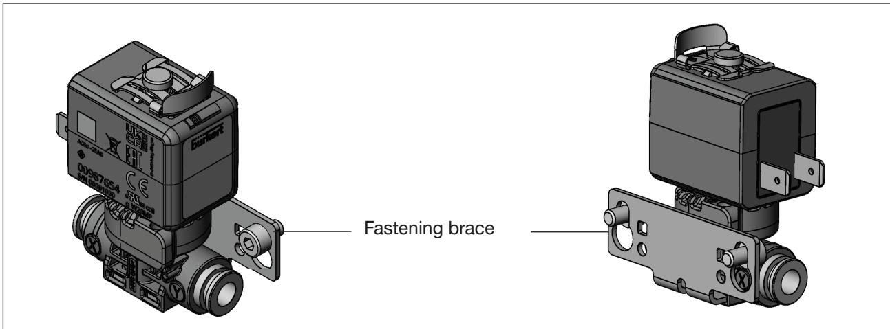
Fig. 6: Installation of devices with a fastening brace
