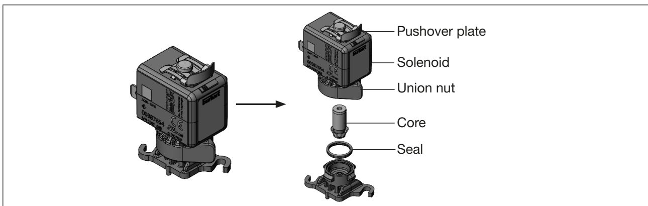
Fig. 10: Wearing parts
