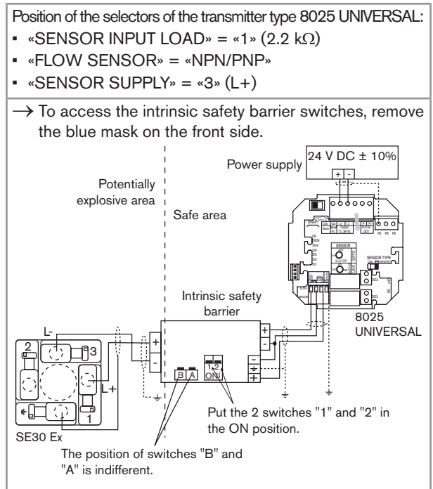
Fig. 7 : Connection between an SE30 Ex and a panel version of the transmitter type 8025 UNIVERSAL
