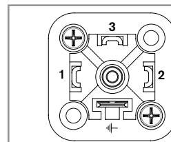
Fig. 3 : Pin assignment of the male connector
