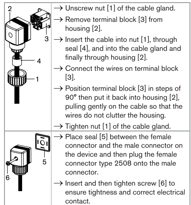
Fig. 4 : Assembling the female connector type 2508 (supplied)
