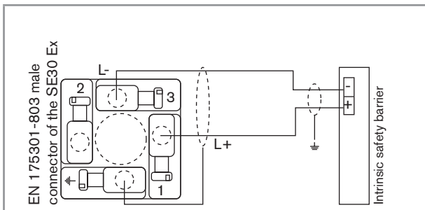
Fig. 5 : Wiring the SE30 Ex to an intrinsic safety barrier
