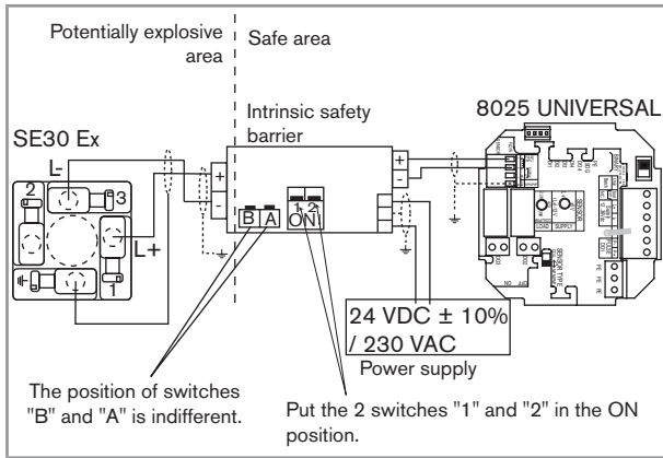
Fig. 6 : Connection between an SE30 Ex and a panel version of the transmitter type 8025 UNIVERSAL
