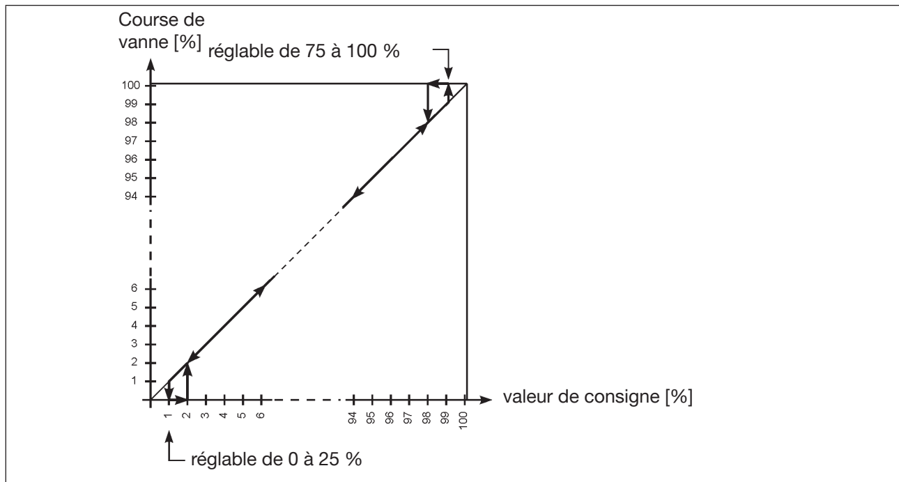
Figure 13 : Diagramme CUTOFF
