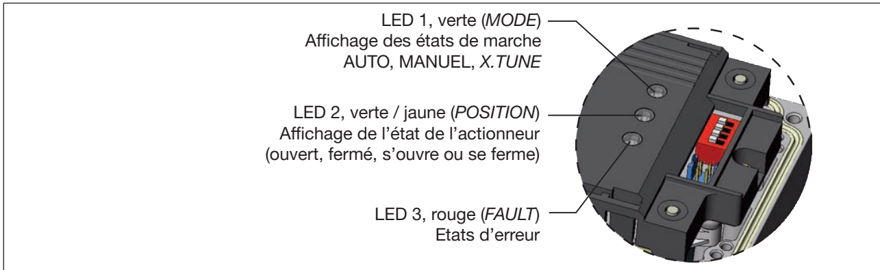
Figure 11 : Affichage LED
