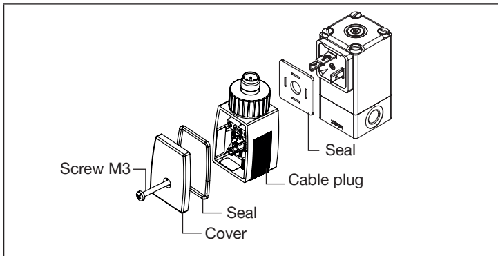
Fig. 4: Mounting the control electronics on the valve
