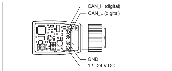
Fig. 2: Terminal strip connection
