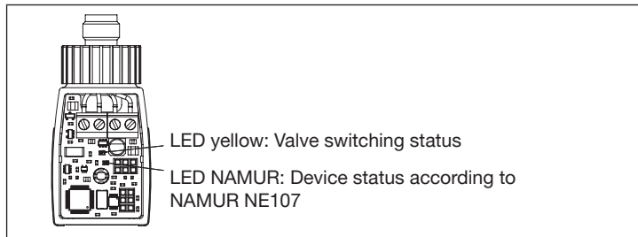
Fig. 5: LED display of the control electronics without an operating unit
