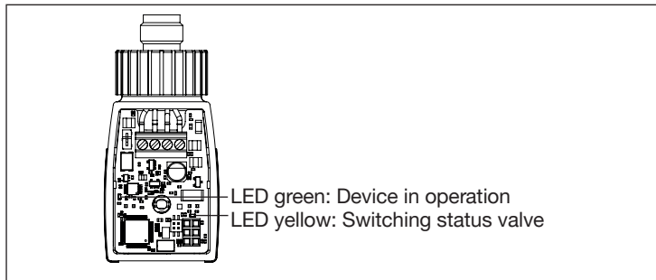
Fig. 6: LEDs for version without operating unit
