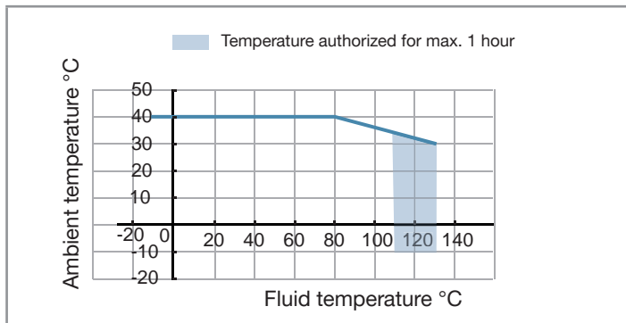
Fig. 2: Fluid temperature depending on the ambient temperature for an ATEX product
