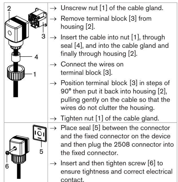
Fig. 2: Assembling the female connector type 2508 (supplied)
