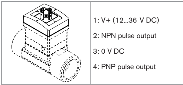
Fig. 3: Pin assignment of the fixed connector, version with pulse outputs
