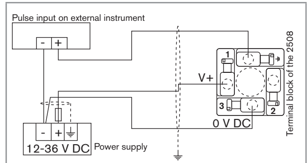
Fig. 5: PNP wiring of the version with pulse outputs
