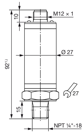
With NPT 1/4" process connection according to EN 837
