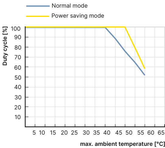
Derating curve for positioner and process controller DN 8...DN 10: see operating instructions Type 3280 ▶.
