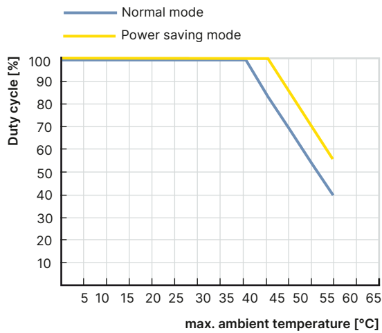
Derating curve for positioner and process controller DN 8...DN 10: see operating instructions Type 3280 ▶.
