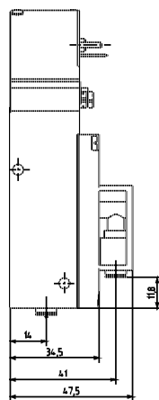
Pict. 6: Plug-in coupling \varnothing 6 mm, below, tag connectors in front
